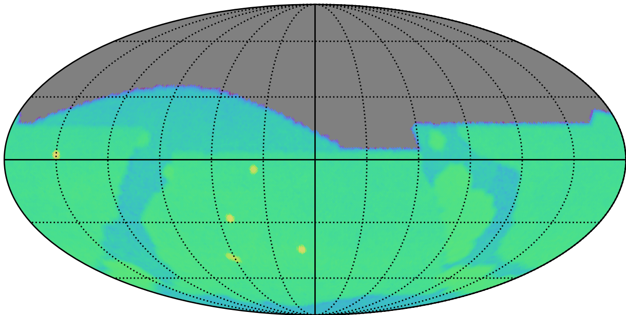
ddf_loaded_half_fl8_v3.4_10yrs g: SurfaceBrightLimit
