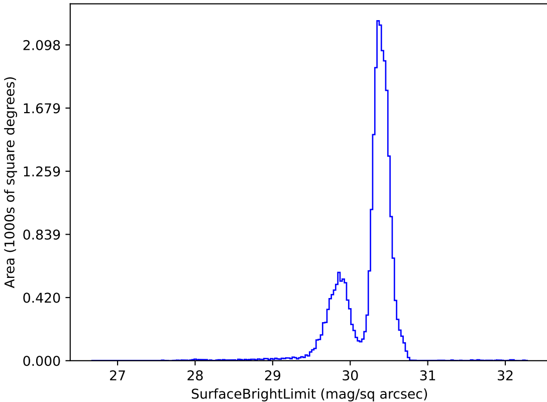
ddf_loaded_half_fl8_v3.4_10yrs g: SurfaceBrightLimit
