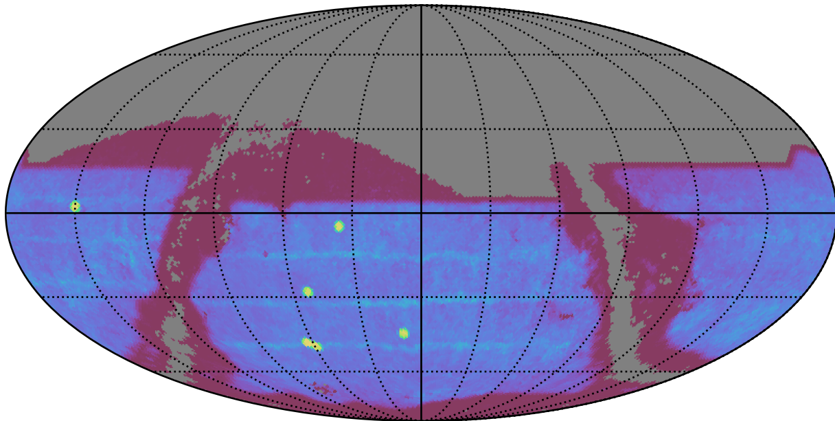
ddf_loaded_half_fl8_v3.4_10yrs : SNSLMetric
