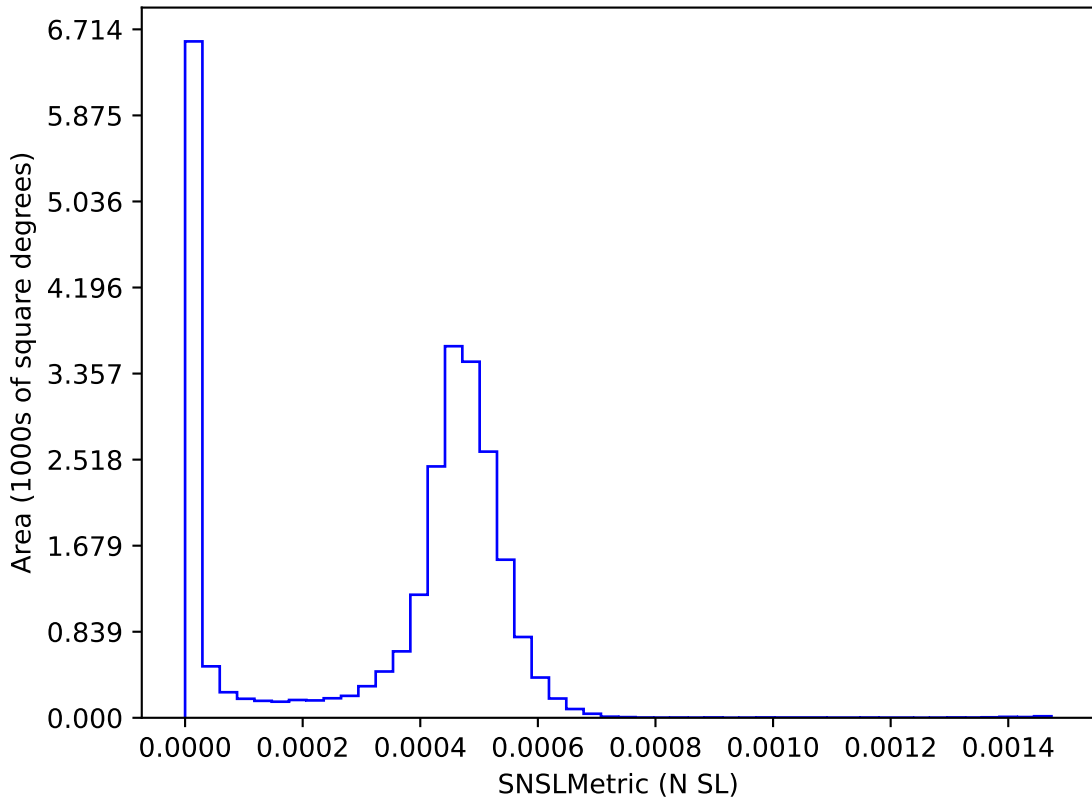
ddf_loaded_half_fl8_v3.4_10yrs : SNSLMetric
