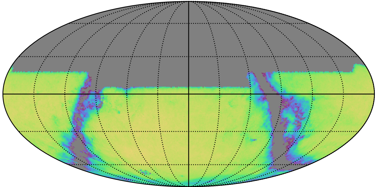
ddf_loaded_half_fl8_v3.4_10yrs u band and non-DD: QSONumberCountsMetric
