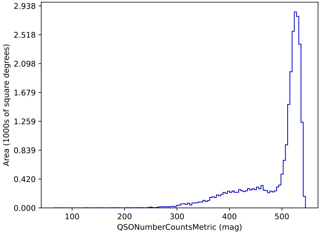
ddf_loaded_half_fl8_v3.4_10yrs r band and non-DD: QSONumberCountsMetric
