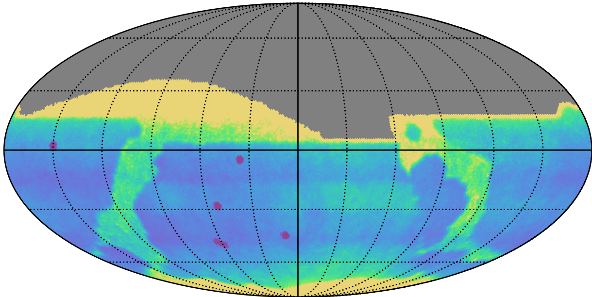
ddf_loaded_half_fl8_v3.4_10yrs : Proper Motion Uncert @ 24.0
