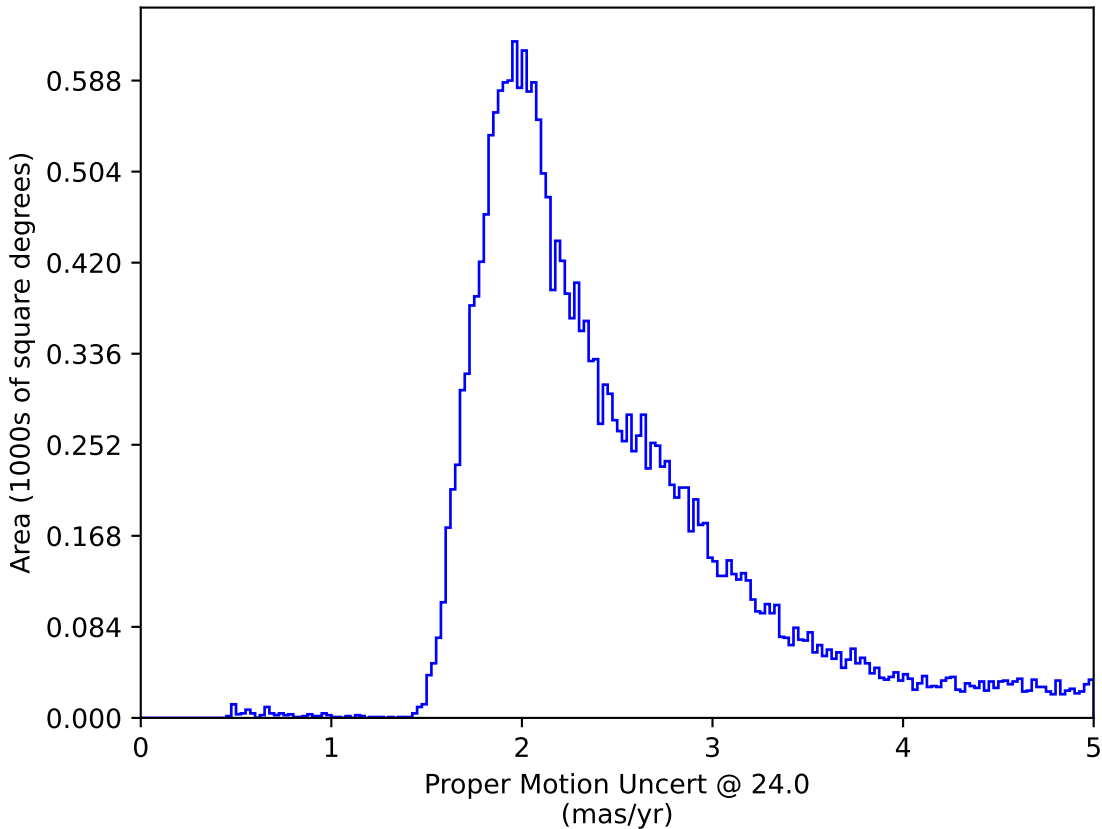
ddf_loaded_half_fl8_v3.4_10yrs : Proper Motion Uncert @ 24.0
