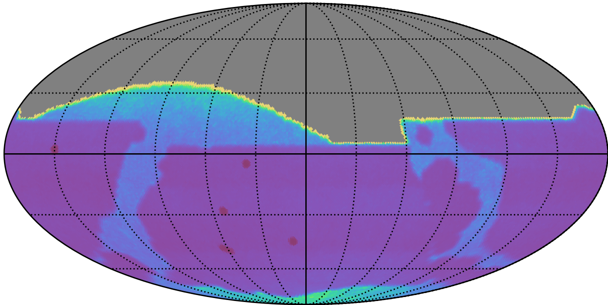
ddf_loaded_half_fl8_v3.4_10yrs : Proper Motion Uncert @ 20.5
