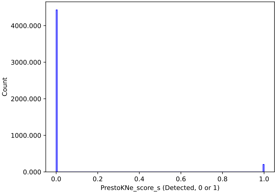
ddf_loaded_half_fl8_v3.4_10yrs : PrestoKNe_score_s
