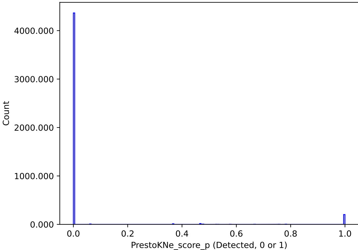
ddf_loaded_half_fl8_v3.4_10yrs : PrestoKNe_score_p
