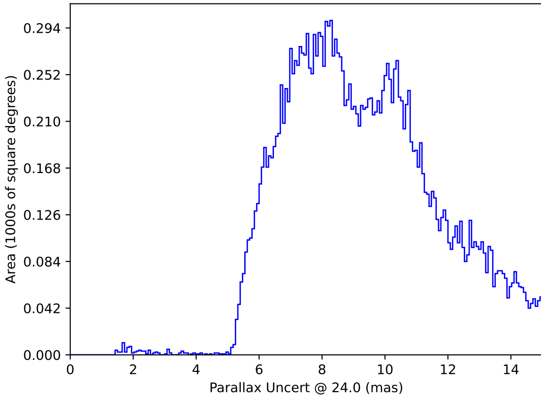
ddf_loaded_half_fl8_v3.4_10yrs : Parallax Uncert @ 24.0
