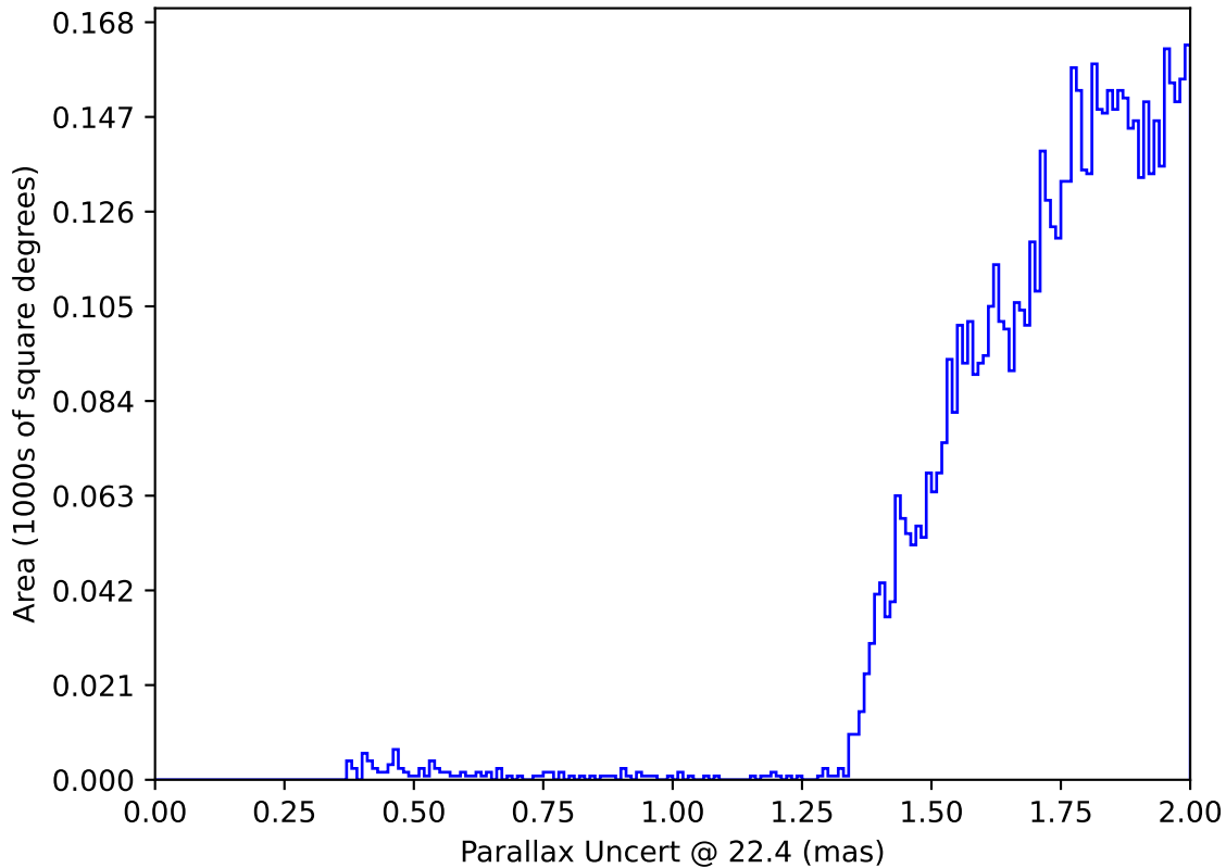
ddf_loaded_half_fl8_v3.4_10yrs : Parallax Uncert @ 22.4
