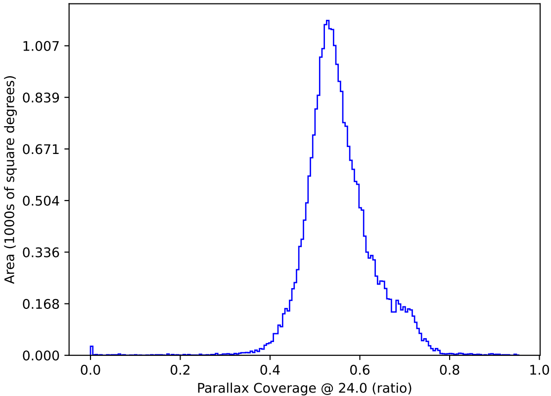
ddf_loaded_half_fl8_v3.4_10yrs : Parallax Coverage @ 24.0
