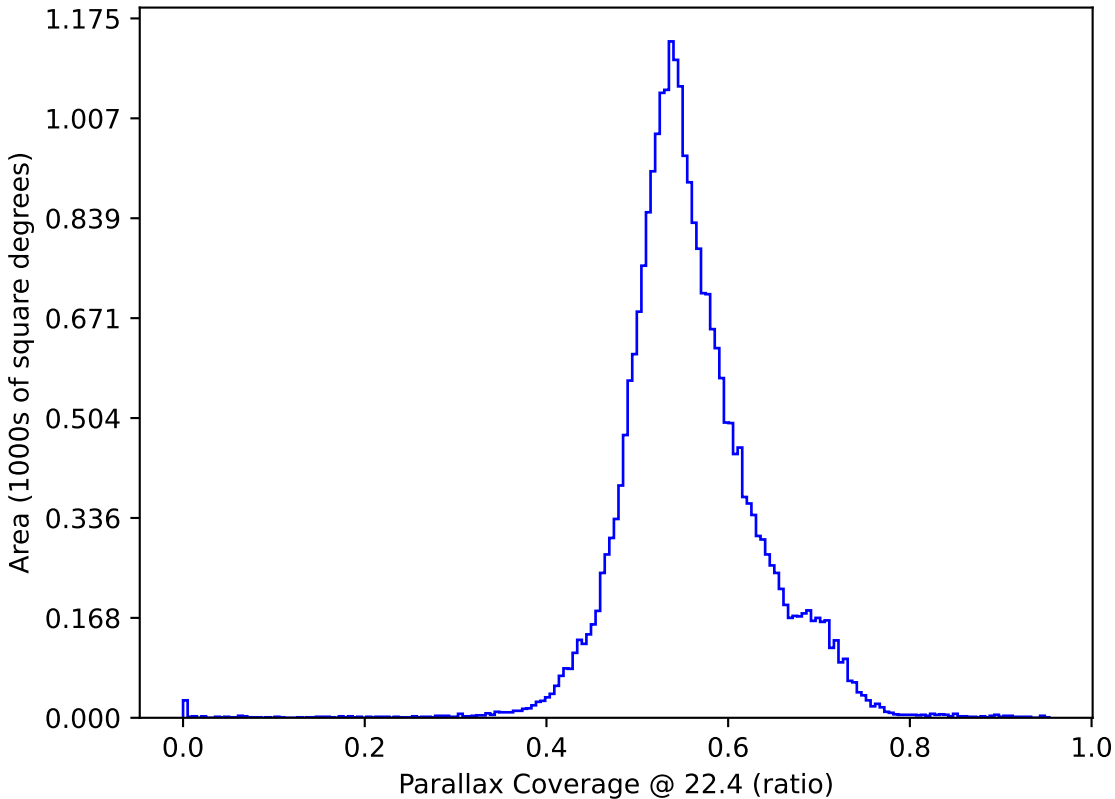
ddf_loaded_half_fl8_v3.4_10yrs : Parallax Coverage @ 22.4
