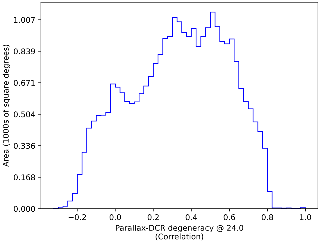
ddf_loaded_half_f18_v3.4_10yrs : Parallax-DCR degeneracy @ 24.0
