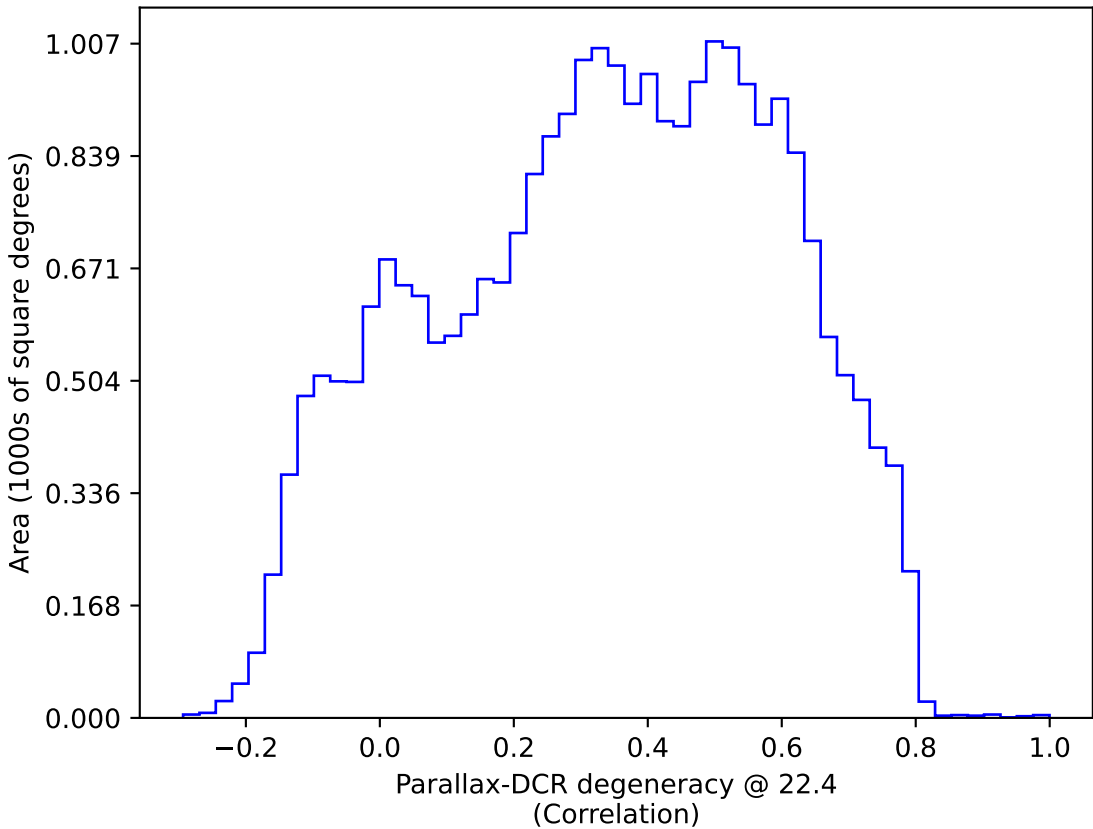
ddf_loaded_half_fl8_v3.4_10yrs : Parallax-DCR degeneracy @ 22.4
