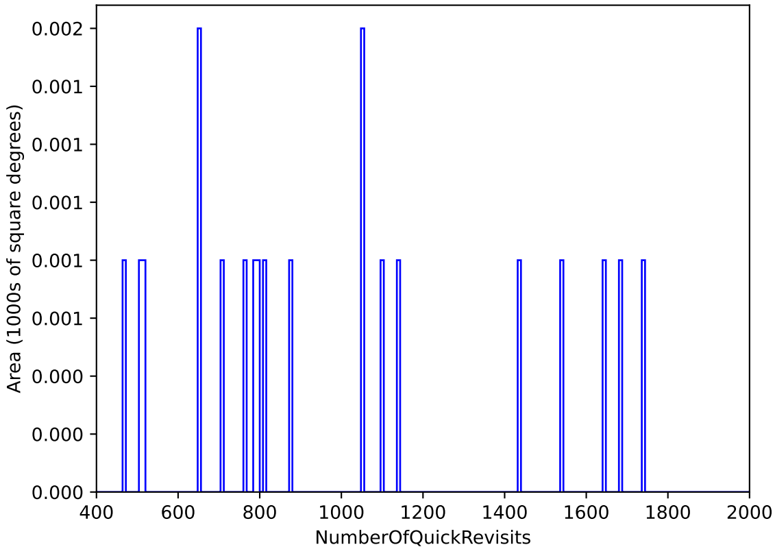
ddf_loaded_half_fl8_v3.4_10yrs : NumberOfQuickRevisits
