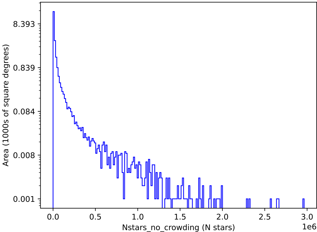
ddf_loaded_half_fl8_v3.4_10yrs u: Nstars_no_crowding
