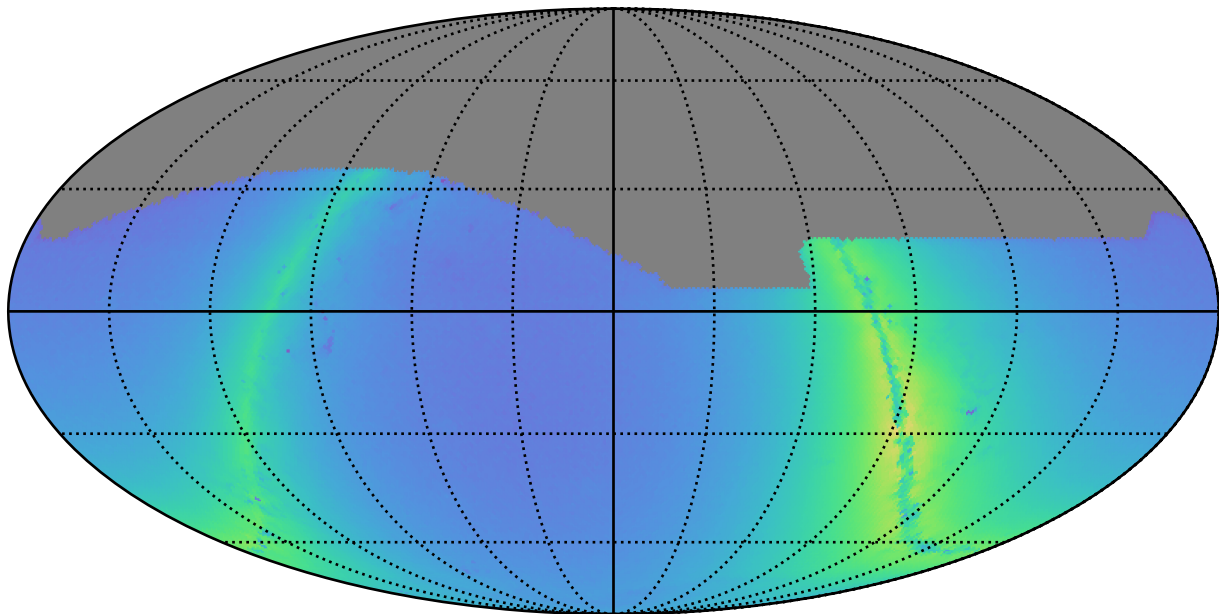
ddf_loaded_half_fl8_v3.4_10yrs r: Nstars_no_crowding
