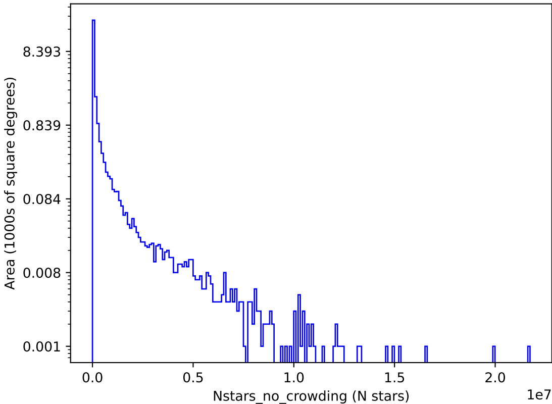
ddf_loaded_half_fl8_v3.4_10yrs r: Nstars_no_crowding
