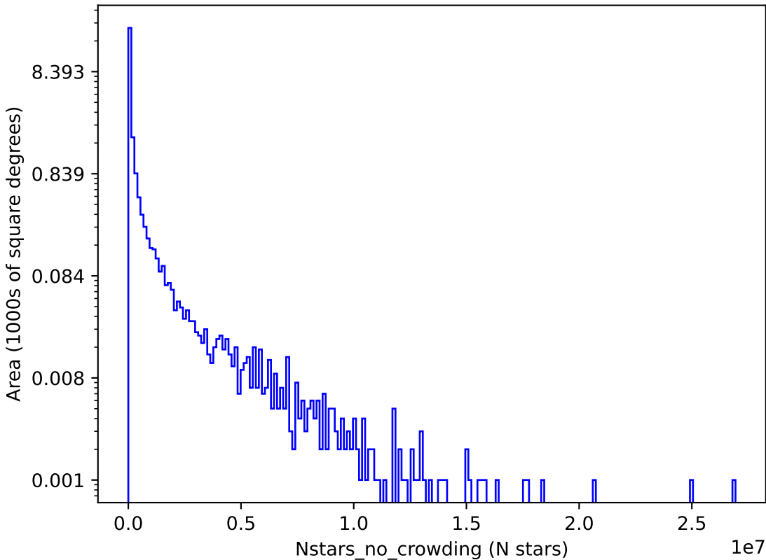
ddf_loaded_half_f18_v3.4_10yrs i: Nstars_no_crowding
