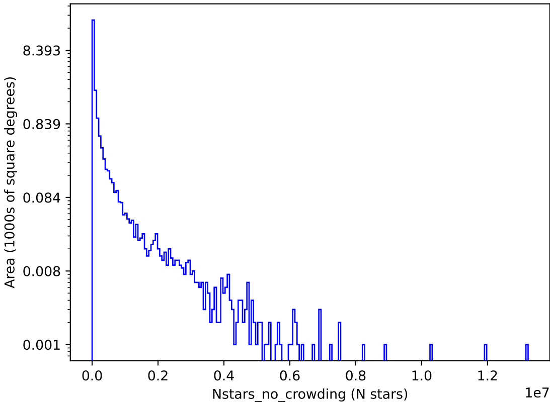
ddf_loaded_half_fl8_v3.4_10yrs g: Nstars_no_crowding
