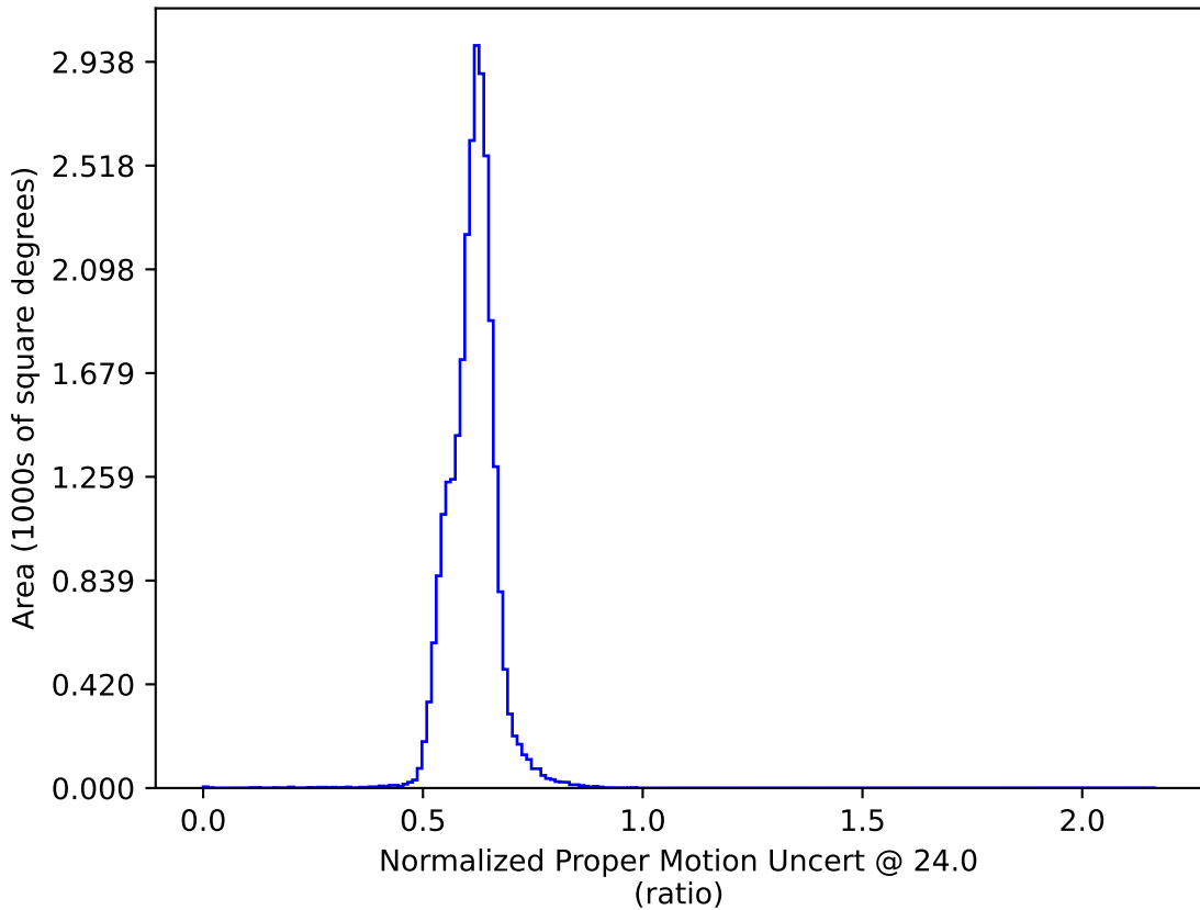
ddf_loaded_half_fl8_v3.4_10yrs : Normalized Proper Motion Uncert @ 24.0
