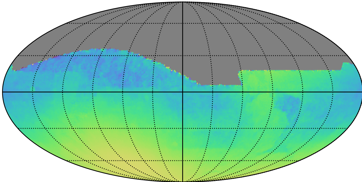
ddf_loaded_half_fl8_v3.4_10yrs : Normalized Parallax Uncert @ 24.0
