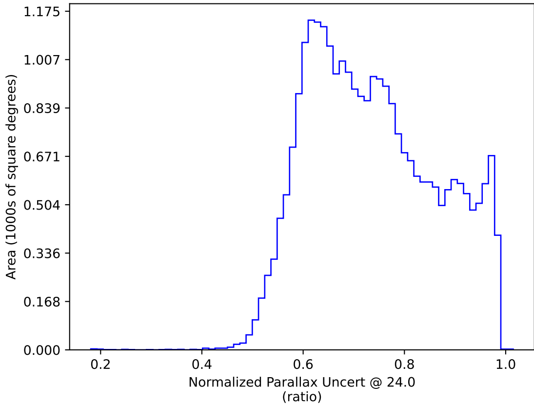
ddf_loaded_half_fl8_v3.4_10yrs : Normalized Parallax Uncert @ 24.0
