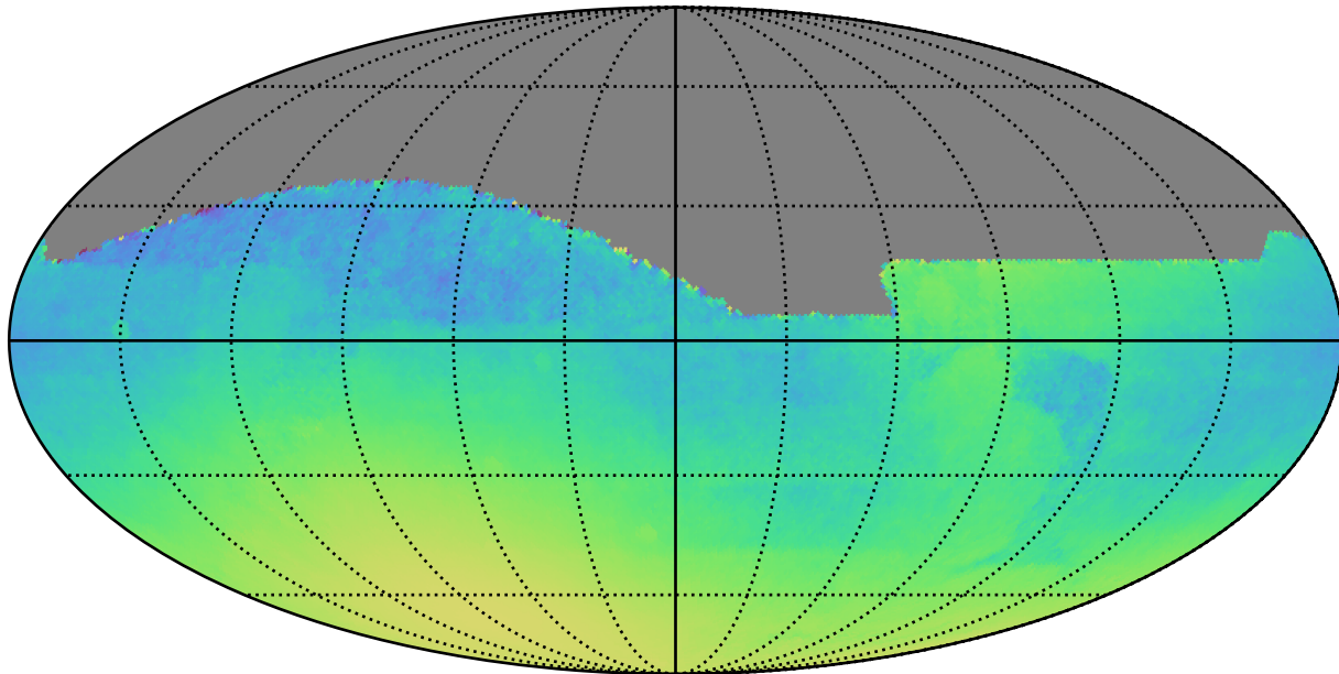
ddf_loaded_half_fl8_v3.4_10yrs : Normalized Parallax Uncert @ 22.4
