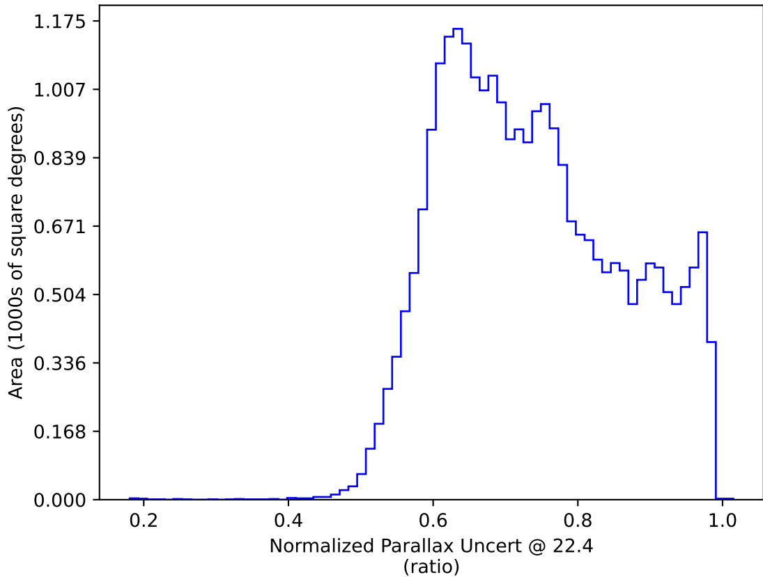
ddf_loaded_half_fl8_v3.4_10yrs : Normalized Parallax Uncert @ 22.4
