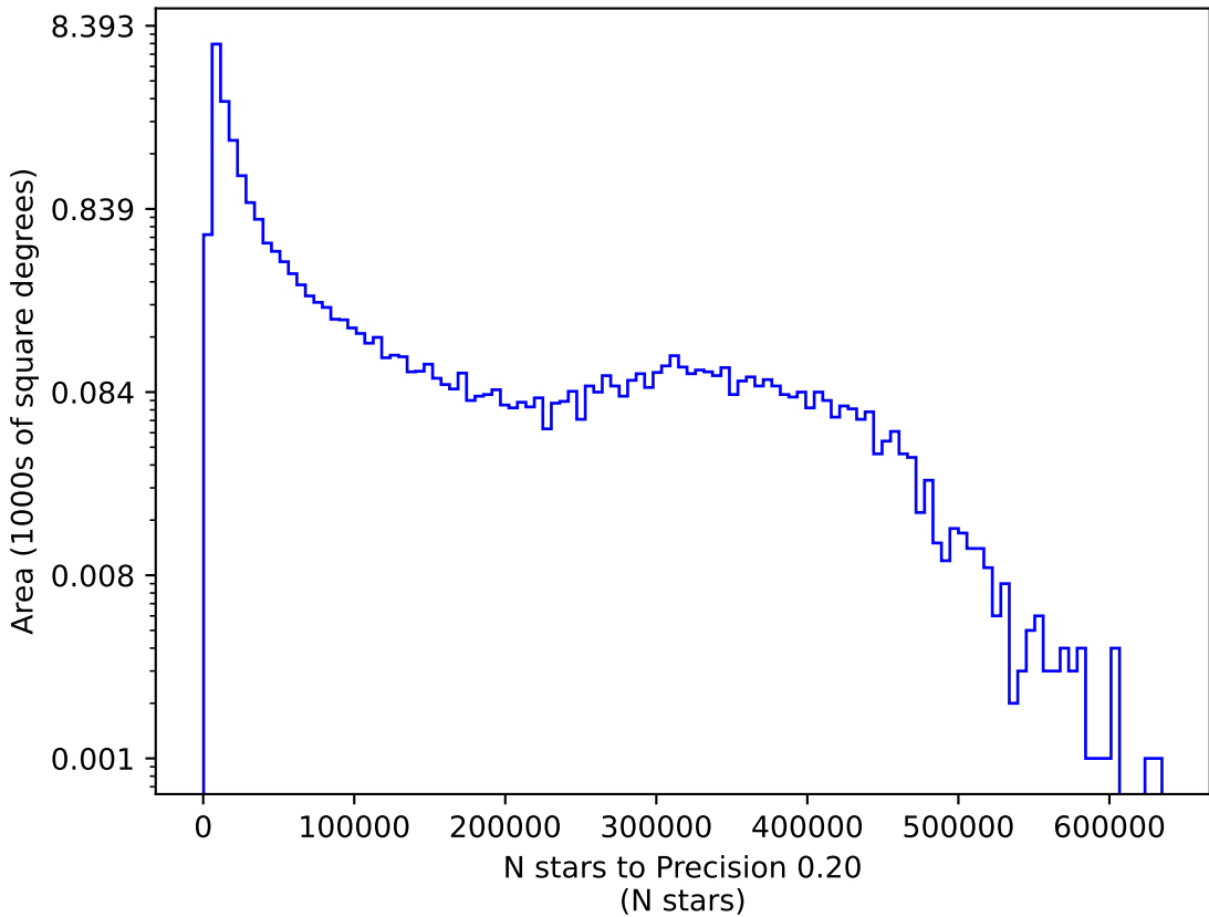
ddf_loaded_half_f18_v3.4_10yrs y: N stars to Precision 0.20
