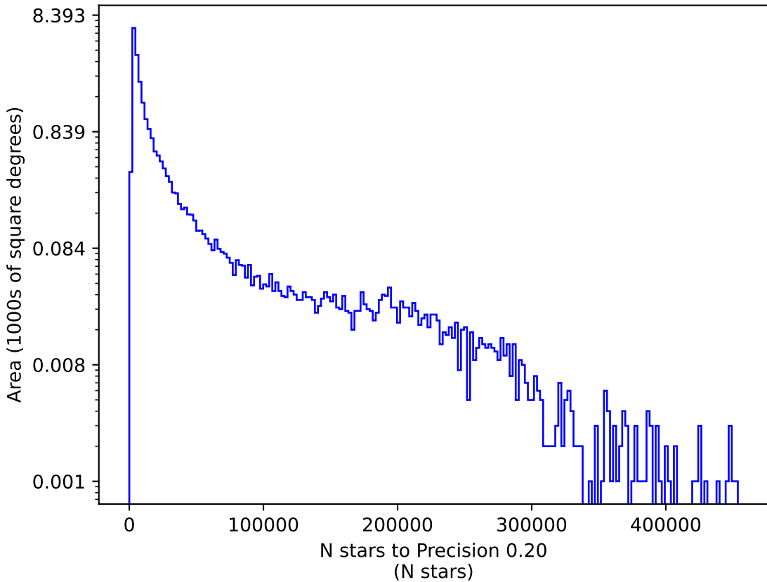
ddf_loaded_half_fl8_v3.4_10yrs u: N stars to Precision 0.20
