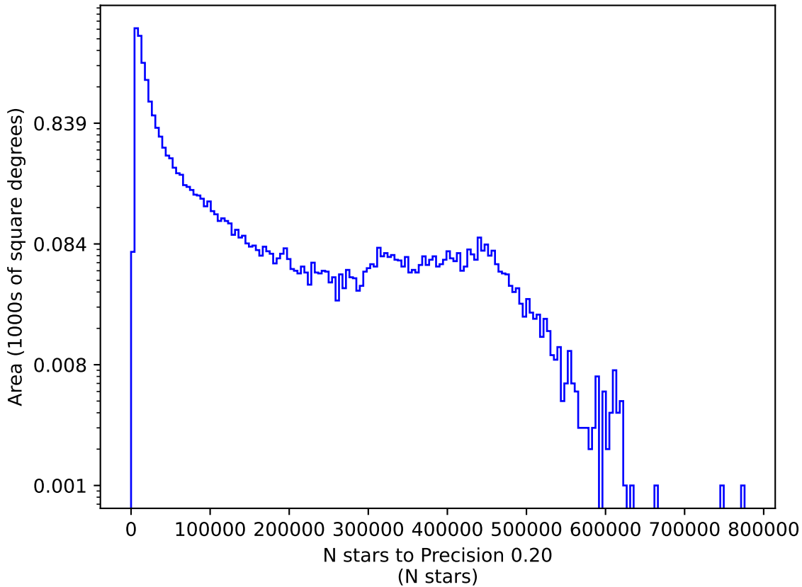
ddf_loaded_half_fl8_v3.4_10yrs r: N stars to Precision 0.20
