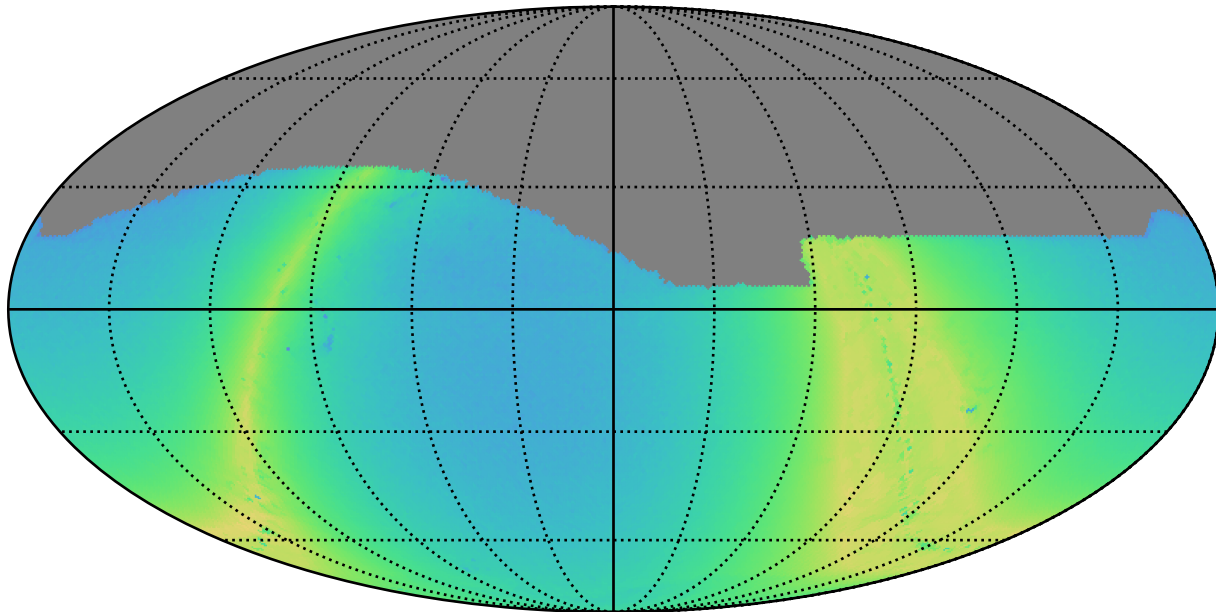
ddf_loaded_half_fl8_v3.4_10yrs i: N stars to Precision 0.20
