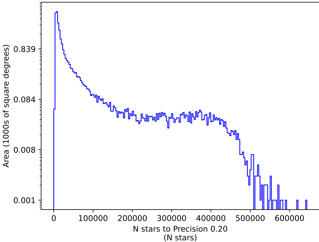
ddf_loaded_half_fl8_v3.4_10yrs g: N stars to Precision 0.20
