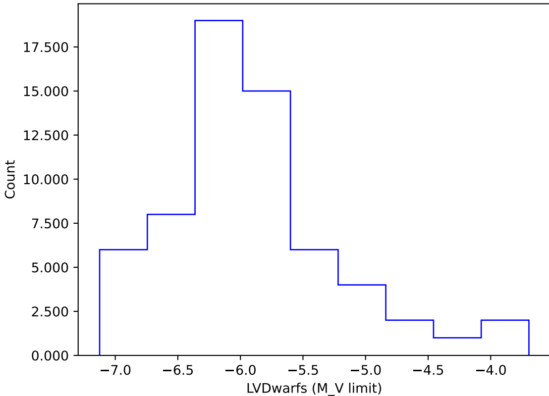
ddf_loaded_half_fl8_v3.4_10yrs gi: LVDwarfs
