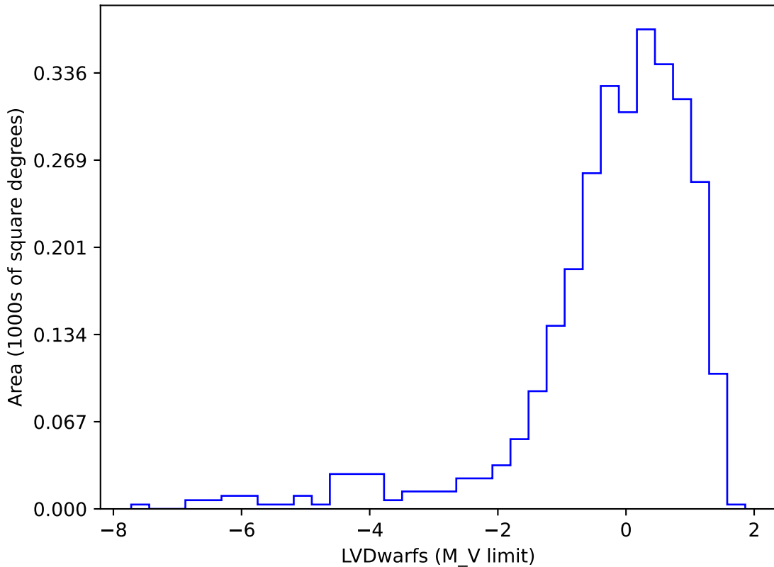
ddf_loaded_half_fl8_v3.4_10yrs gi SCP: LVDwarfs
