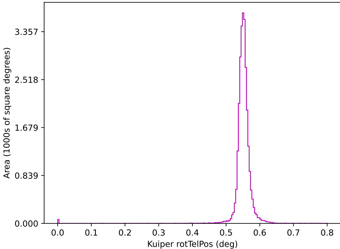
ddf_loaded_half_fl8_v3.4_10yrs z: Kuiper rotTelPos
