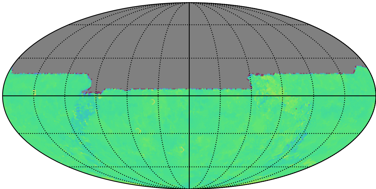
ddf_loaded_half_fl8_v3.4_10yrs u: Kuiper rotTelPos
