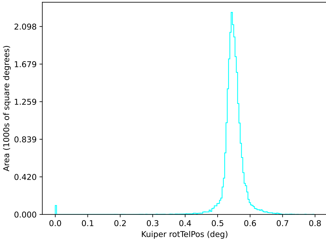
ddf_loaded_half_f18_v3.4_10yrs u: Kuiper rotTelPos
