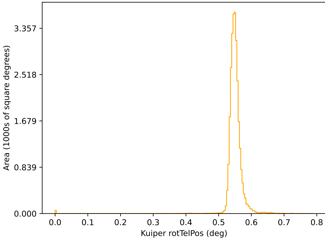
ddf_loaded_half_fl8_v3.4_10yrs r: Kuiper rotTelPos
