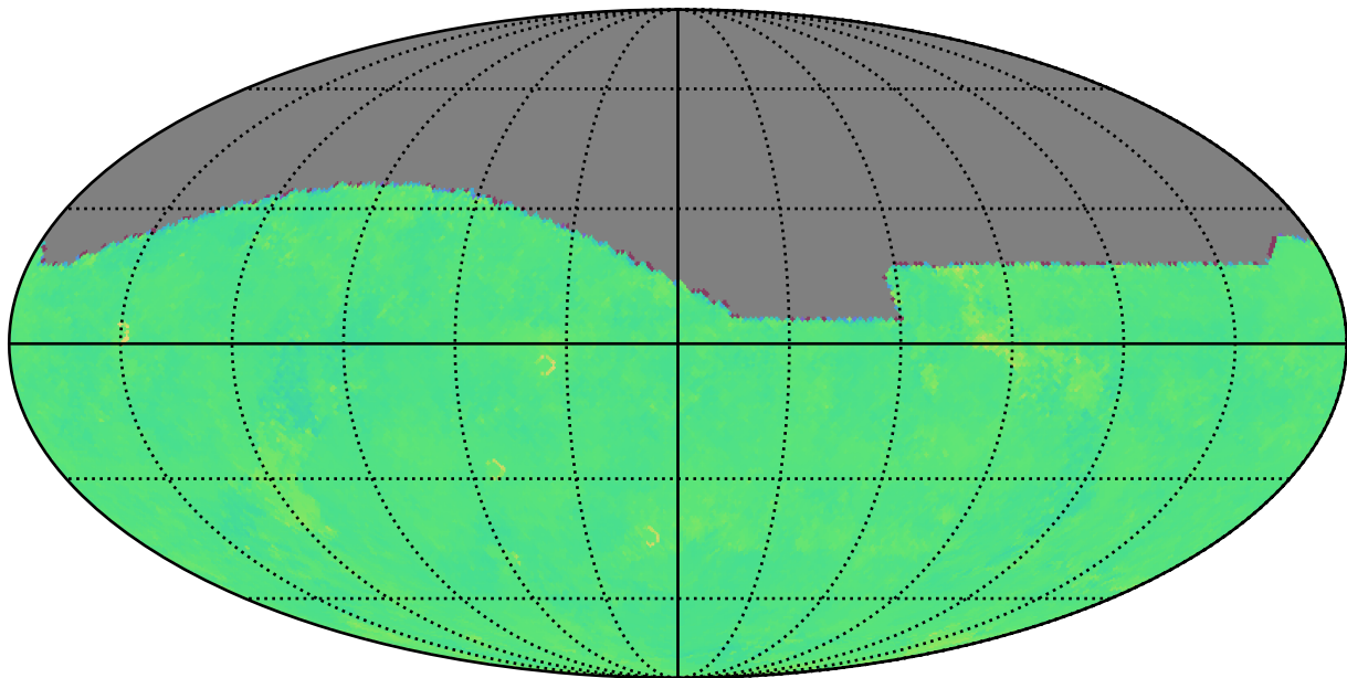
ddf_loaded_half_fl8_v3.4_10yrs g: Kuiper rotTelPos
