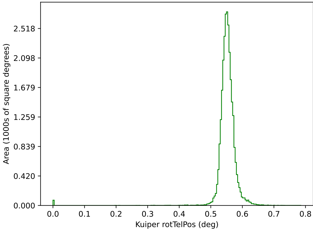
ddf_loaded_half_f18_v3.4_10yrs g: Kuiper rotTelPos
