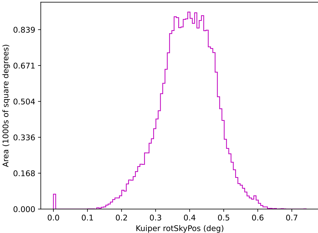
ddf_loaded_half_fl8_v3.4_10yrs z: Kuiper rotSkyPos
