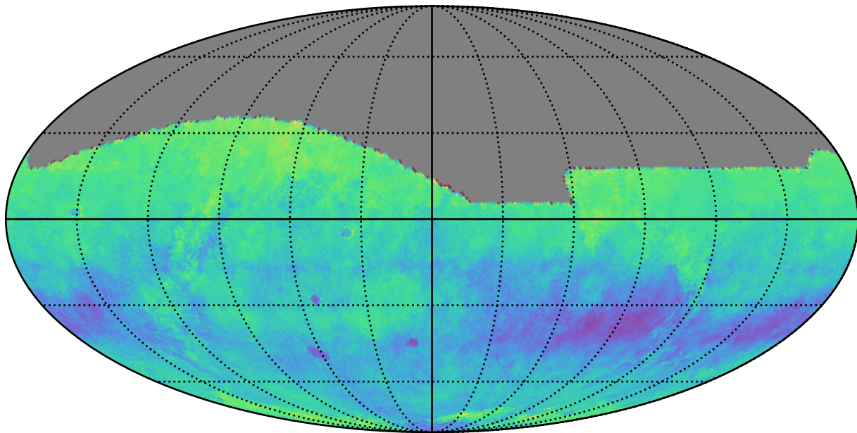
ddf_loaded_half_fl8_v3.4_10yrs r: Kuiper rotSkyPos
