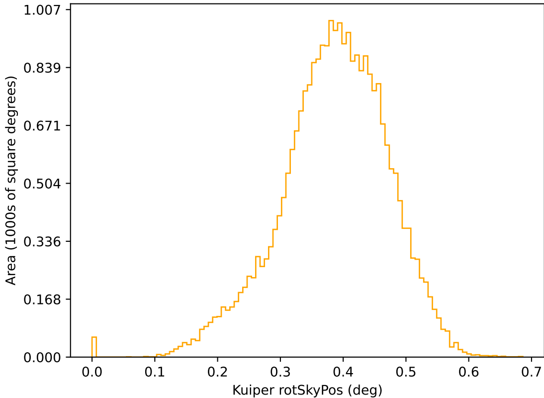
ddf_loaded_half_fl8_v3.4_10yrs r: Kuiper rotSkyPos
