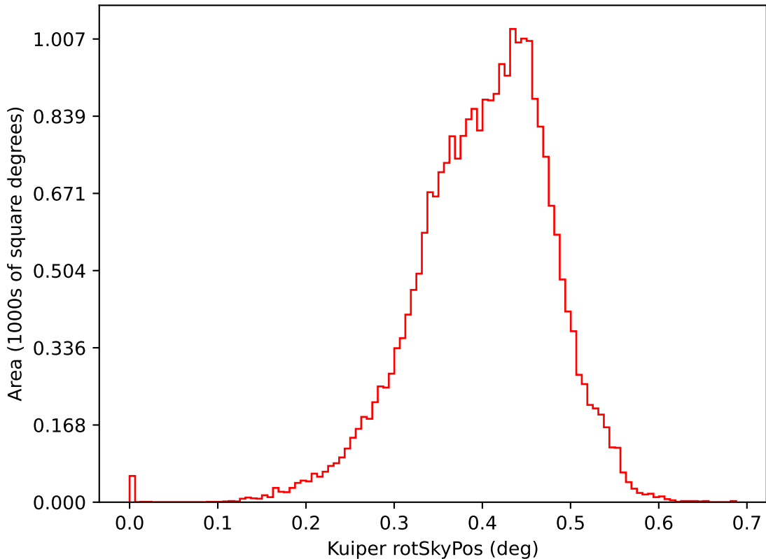
ddf_loaded_half_fl8_v3.4_10yrs i: Kuiper rotSkyPos
