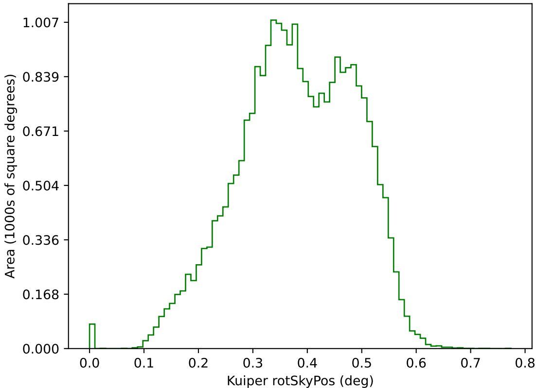
ddf_loaded_half_fl8_v3.4_10yrs g: Kuiper rotSkyPos
