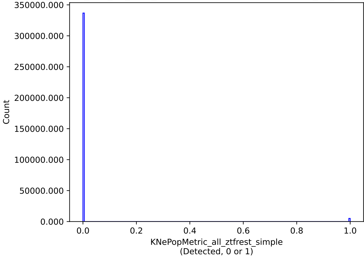
ddf_loaded_half_fl8_v3.4_10yrs all models: KNePopMetric_all_ztfrest_simple
