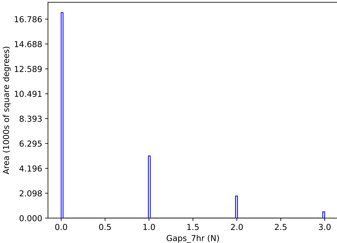
ddf_loaded_half_fl8_v3.4_10yrs y band: Gaps_7hr
