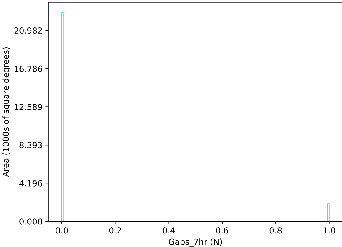
ddf_loaded_half_fl8_v3.4_10yrs u band: Gaps_7hr
