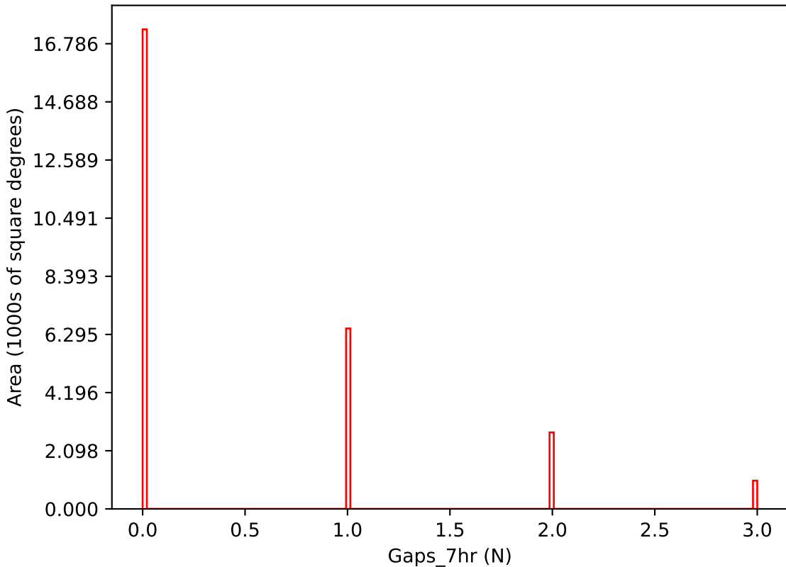
ddf_loaded_half_fl8_v3.4_10yrs i band: Gaps_7hr
